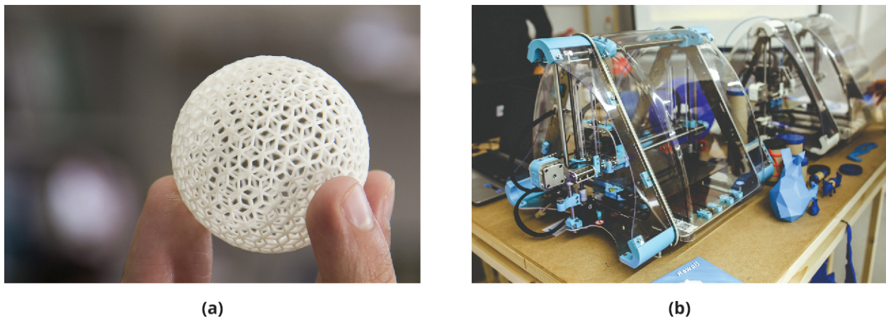
Figure 14.12 3-D printing allows companies to develop prototypes quickly before investing substantial resources. (a) A 3-D sphere, for example, can be created using (b) a 3-D printer. (credit (a): modification of “ball 3d printing design” by “metalurgiamontemar0”/Pixabay, CC0; credit (b): modification of “3d printer printing technology” by “kaboompics”/Pixabay, CC0)
